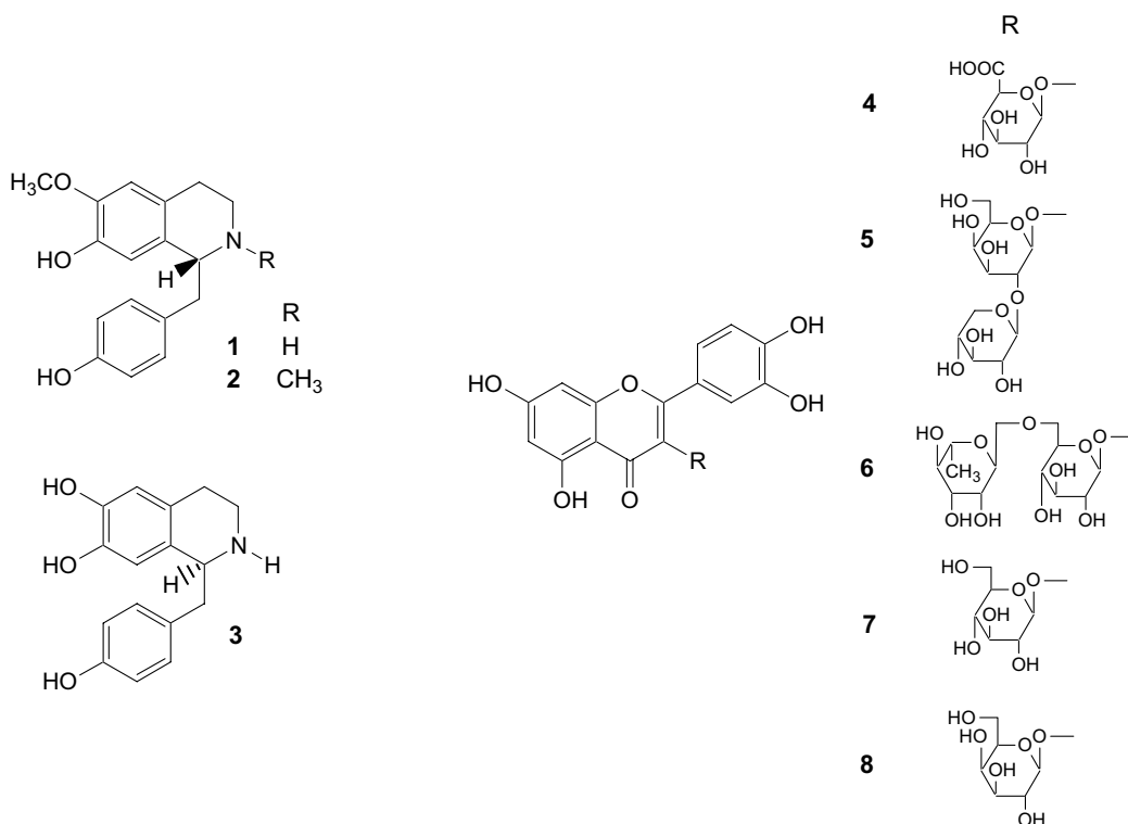
Figure 1. Structures of alkaloids ( 1–3 ) and flavonoids ( 4–8 ) isolated from the leaves of N. nucifera .
