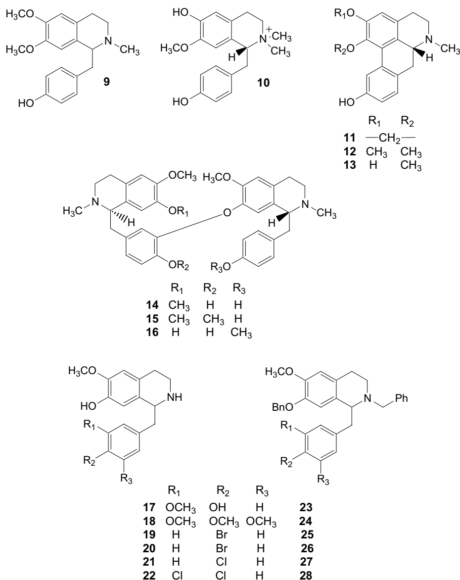
Figure 2. Structures for coclaurine related alkaloids of N. nucifera ( 9–16 ) and synthesized benzylisoquinoline alkaloids ( 17–28 ).
